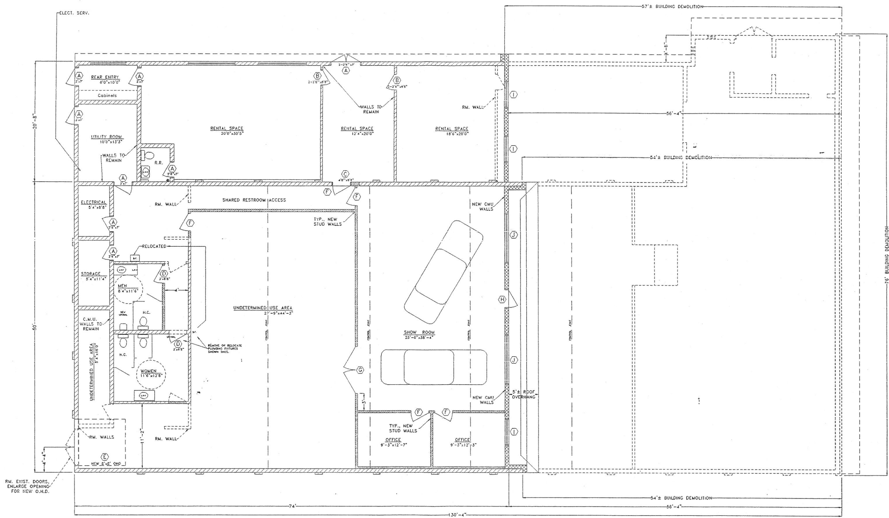
FLOOR PLAN
